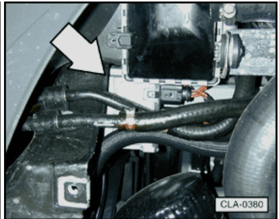
J293 Coolant FC (Fan Control) Control Module (through m.y. 2001)
