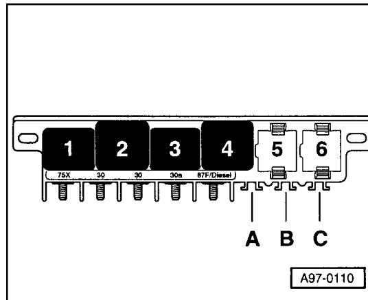
Micro Central Electric Panel behind the storage – driver's side (m.y. 2002)
