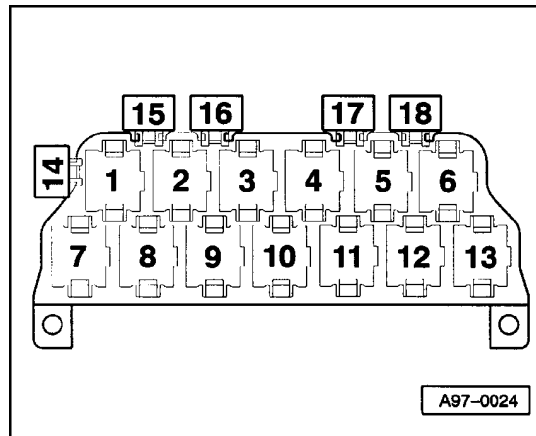
13-Fold Relay Panel behind the storage – driver's side (m.y. 2002)
