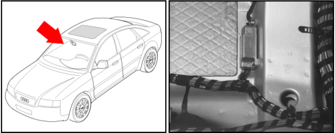
G180 Crash sensor for side airbag, passenger's side
