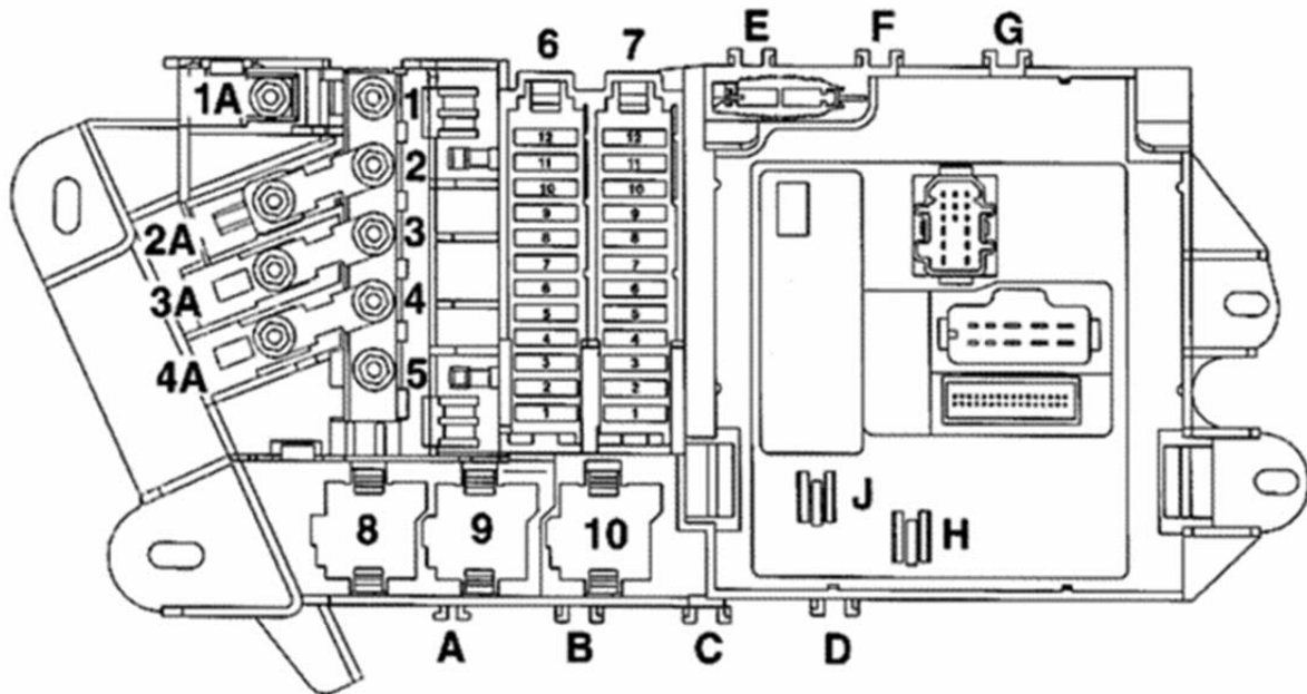
Fig. 19: Fuse Panel (SF) Luggage Compartment - Right Side Courtesy of AUDI OF AMERICA, INC.
