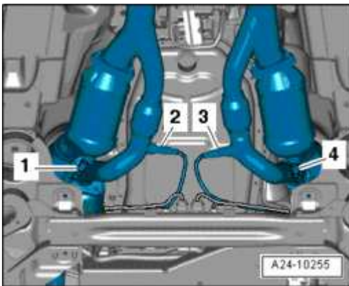
Fig. 16: Oxygen Sensors Courtesy of VOLKSWAGEN UNITED STATES, INC.
