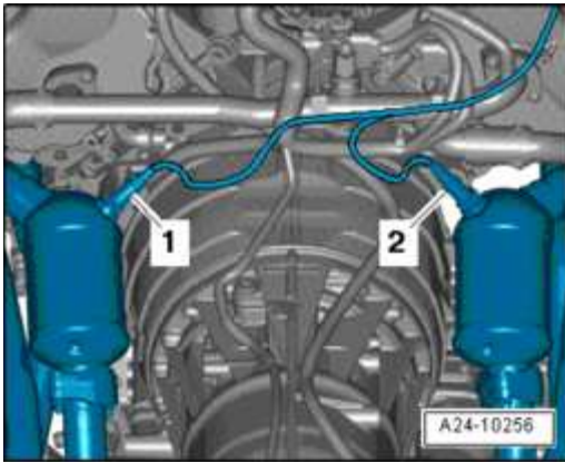
Fig. 15: Oxygen Sensors Before Catalytic Converter Courtesy of VOLKSWAGEN UNITED STATES, INC.
