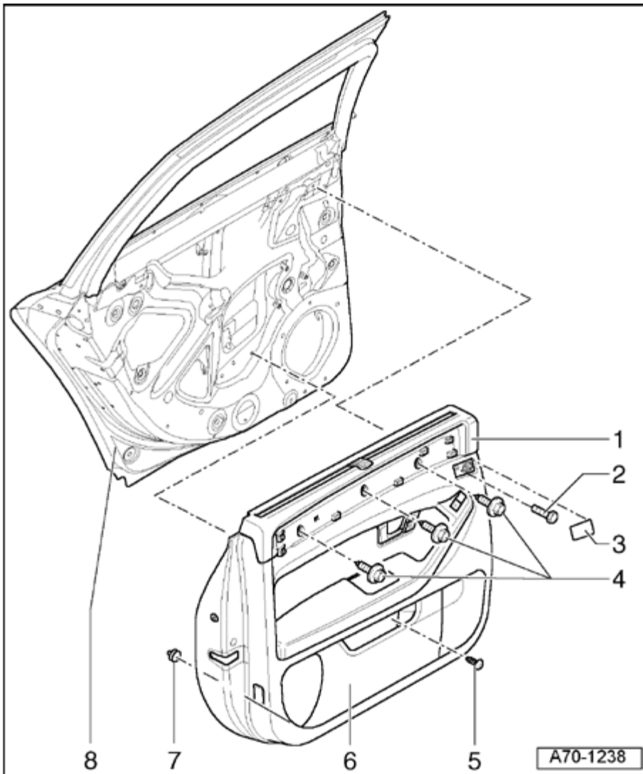
Fig. 398: Rear Door Trim Remove/Install Components Courtesy of VOLKSWAGEN UNITED STATES, INC.
