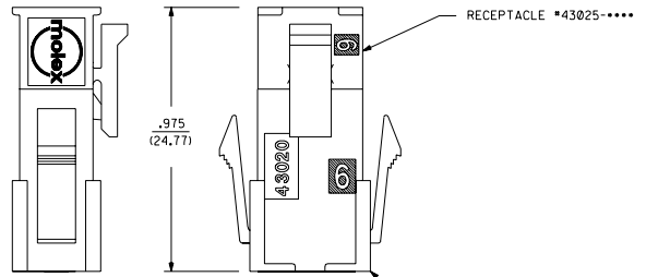
MATED MICRO-FIT CONNECTOR
